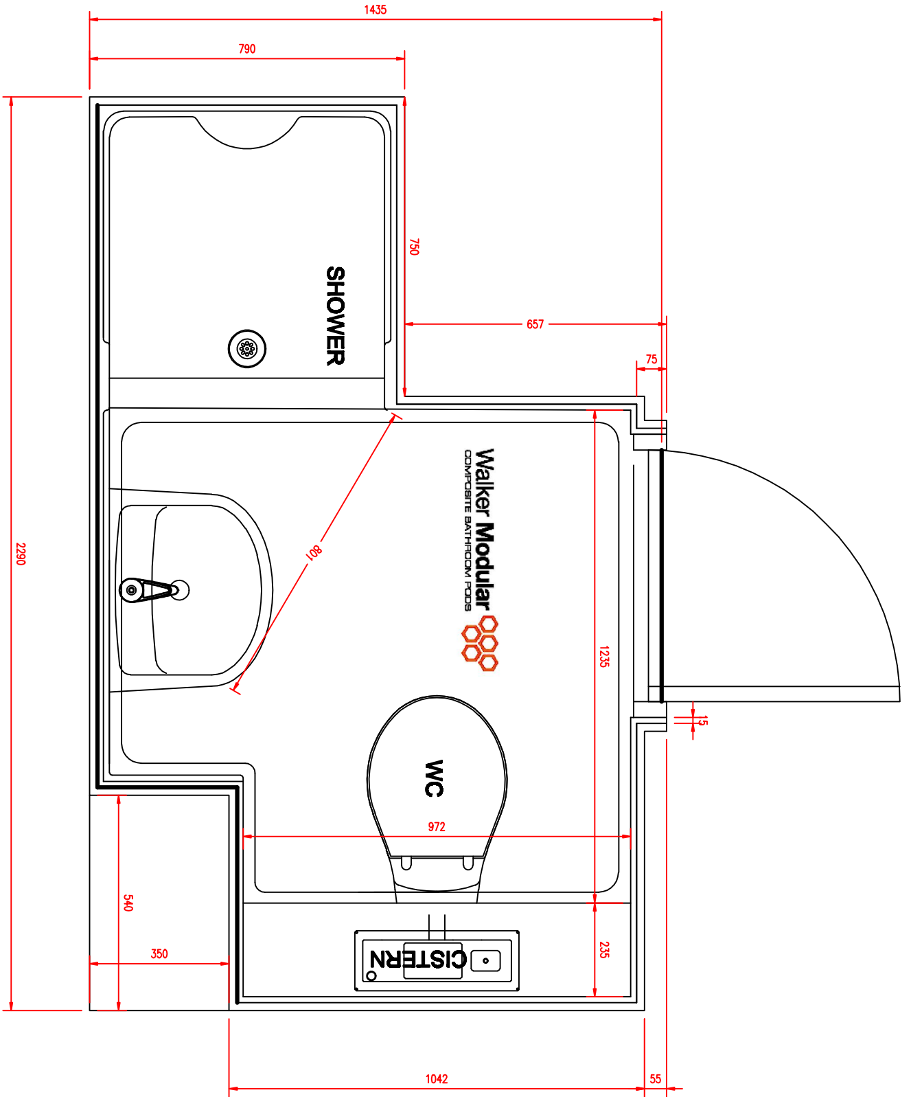
WALKER MODULAR S3 BATHROOM POD PLAN VIEW
